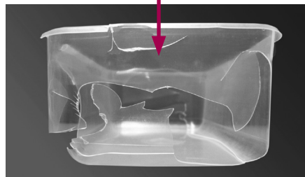
Unmodified container with brittle fracture after impact
