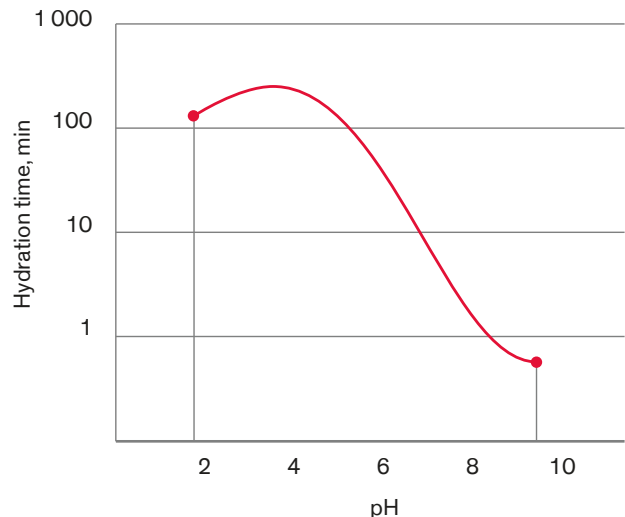
Hydration Delay Time of Surface-Treated METHOCEL™ Products as a Function of pH
