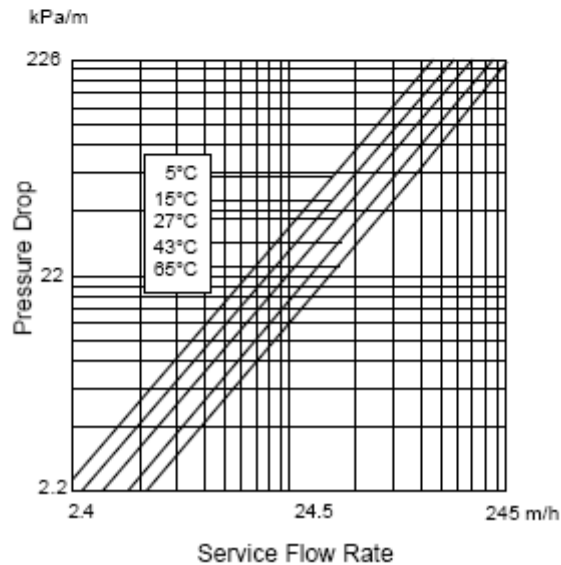
Figure 5 : Pressure Drop
