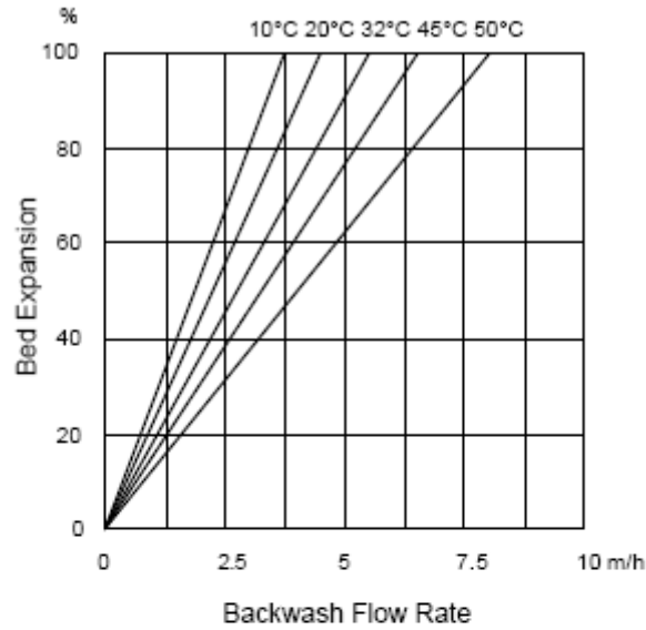
Figure 4 : Bed Expansion
