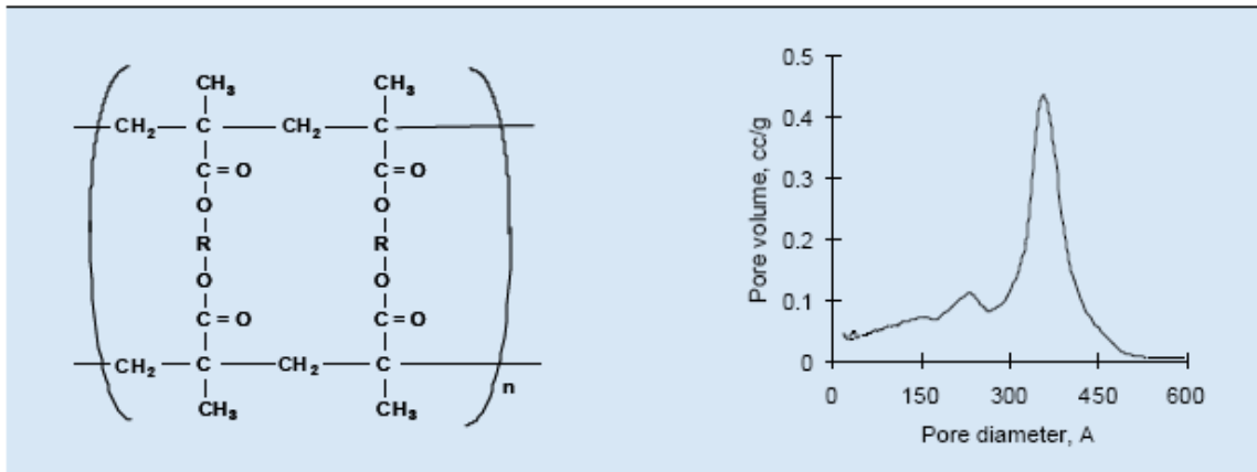
Figure 1 : Chemical structure of AMBERLITE XAD7HP polymeric adsorbent
